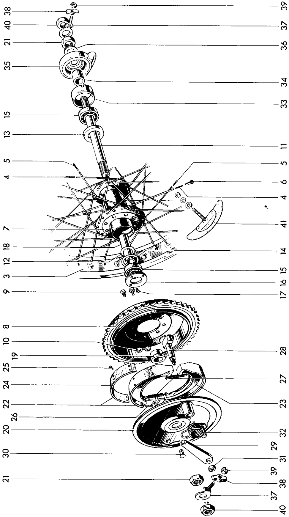
Fig. 18. REAR WHEEL
