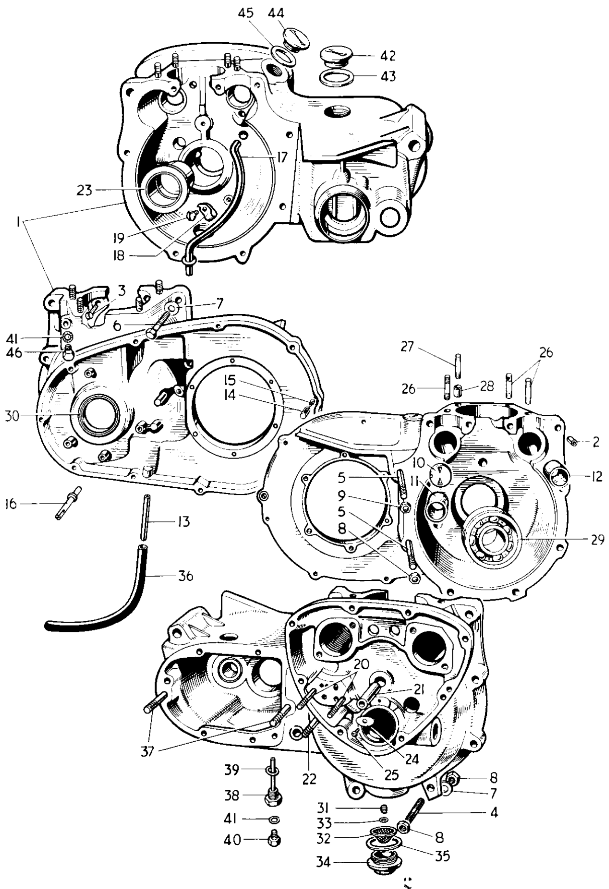
Fig 2. CRANKCASE
