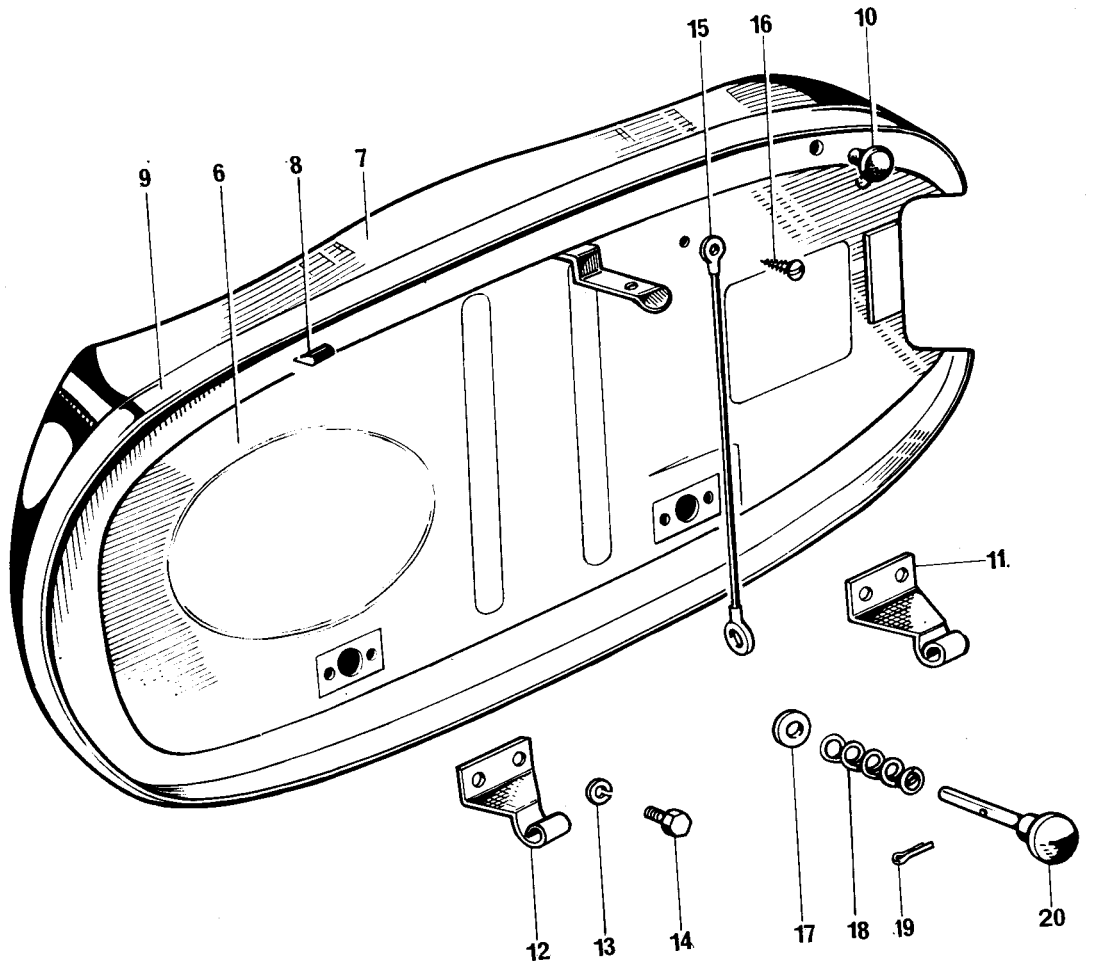
Fig. 26. PANELS AND TWINSEAT
