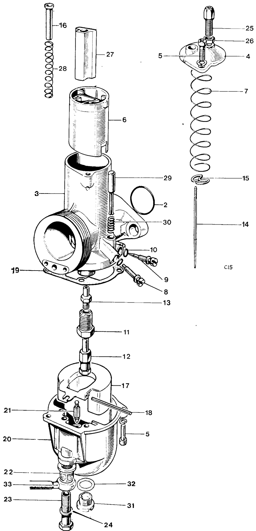
Fig. 6. CARBURETOR, T100R
