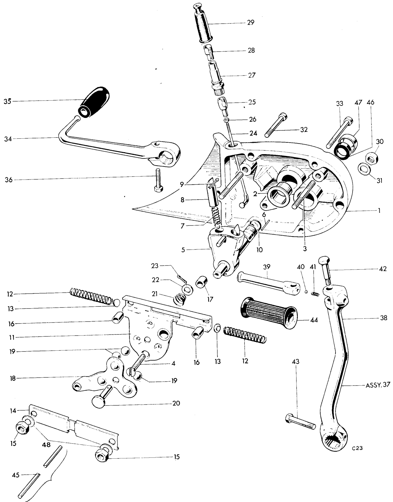
Fig. 12. GEARBOX OUTER COVER AND LEVERS
