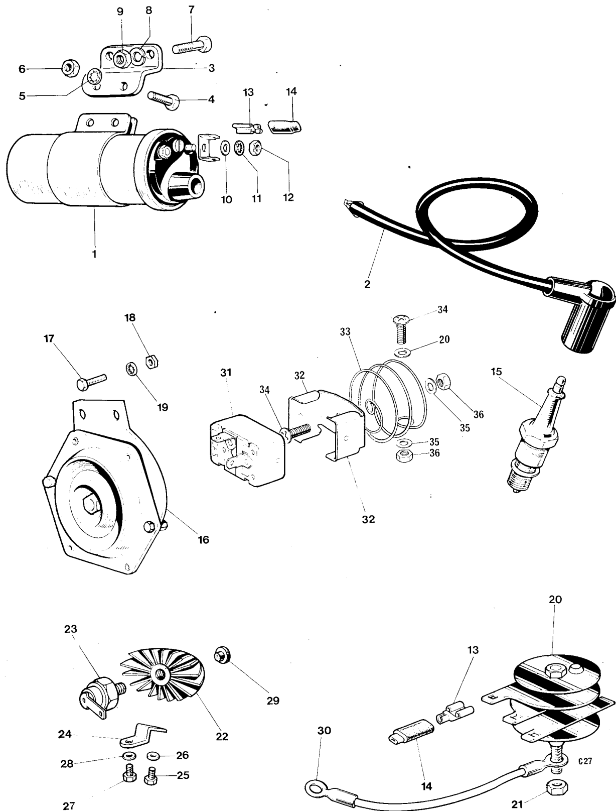
Fig. 33. IGNITION COILS, HORN, RECTIFIER AND ZENER DIODE
