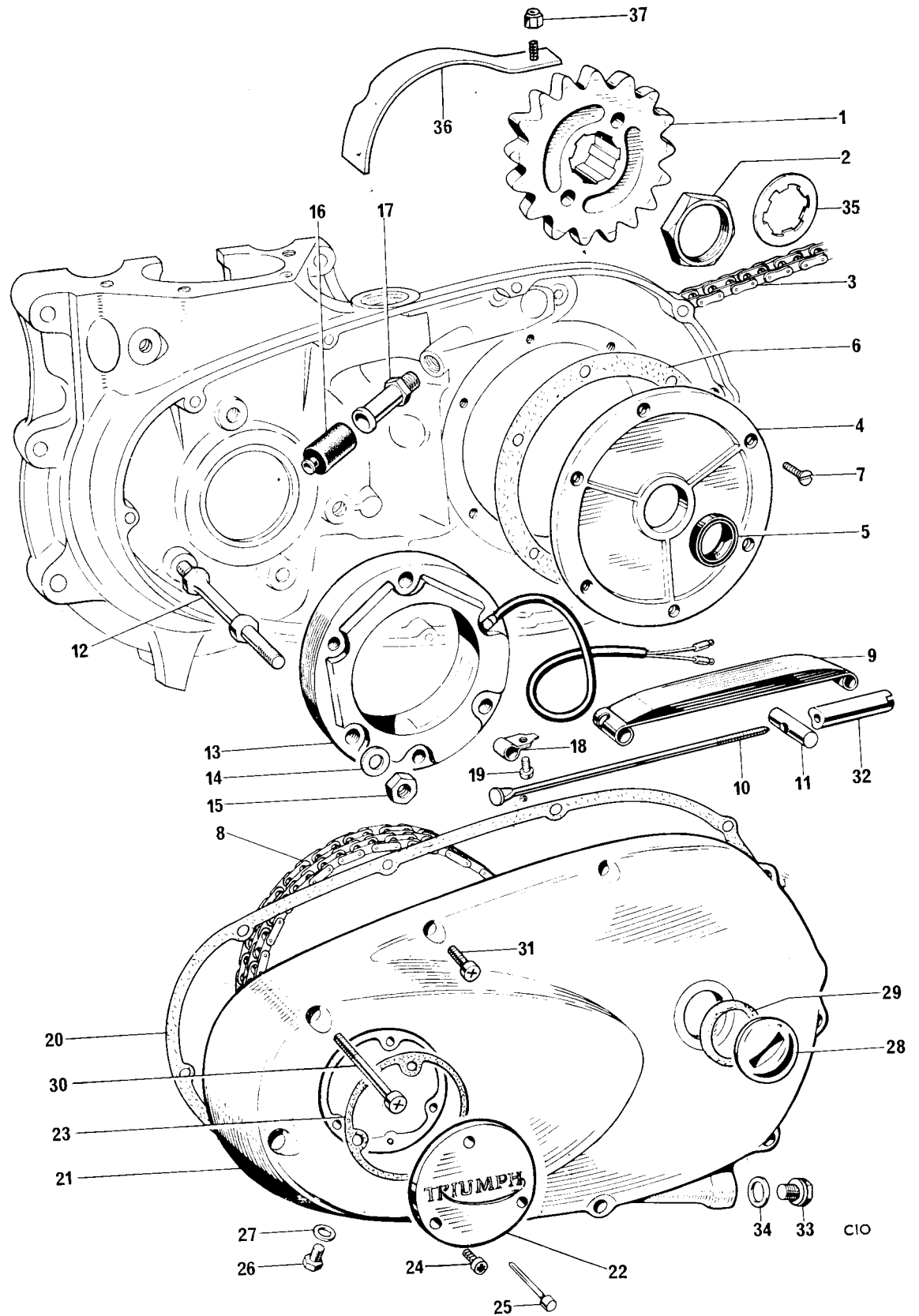
Fig. 14. CHAINCASE AND CHAINS
