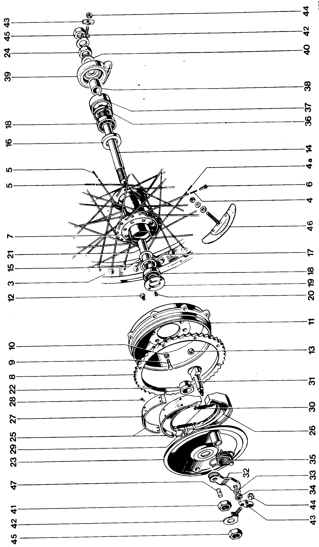
Fig. 23. REAR WHEEL
