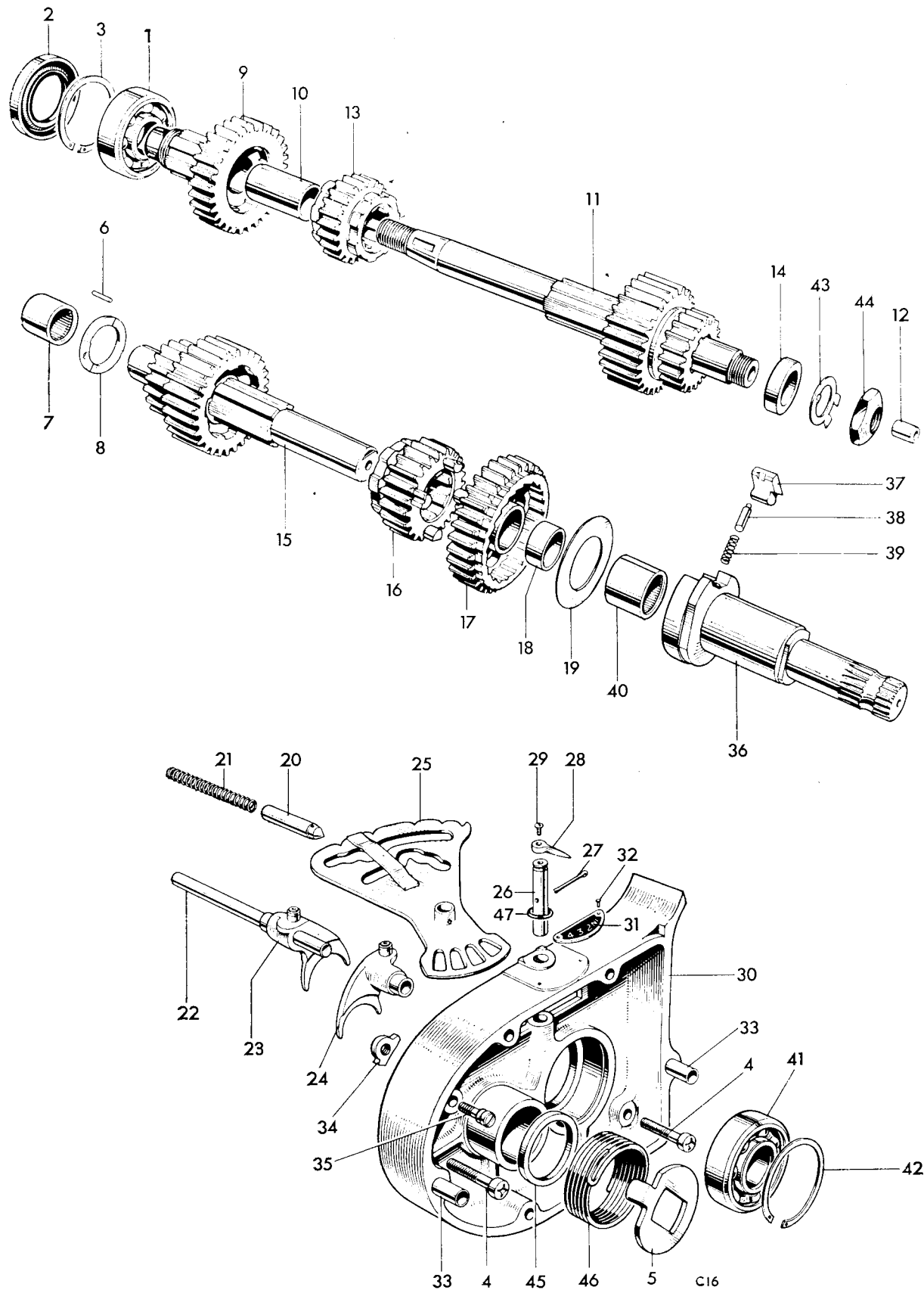
Fig. 11. GEARBOX SHAFTS, BEARINGS AND INNER COVER
