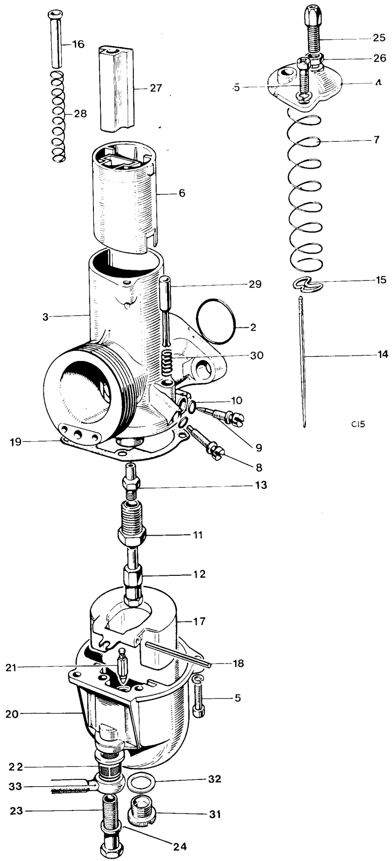
Fig. 5. CARBURETOR T100C
