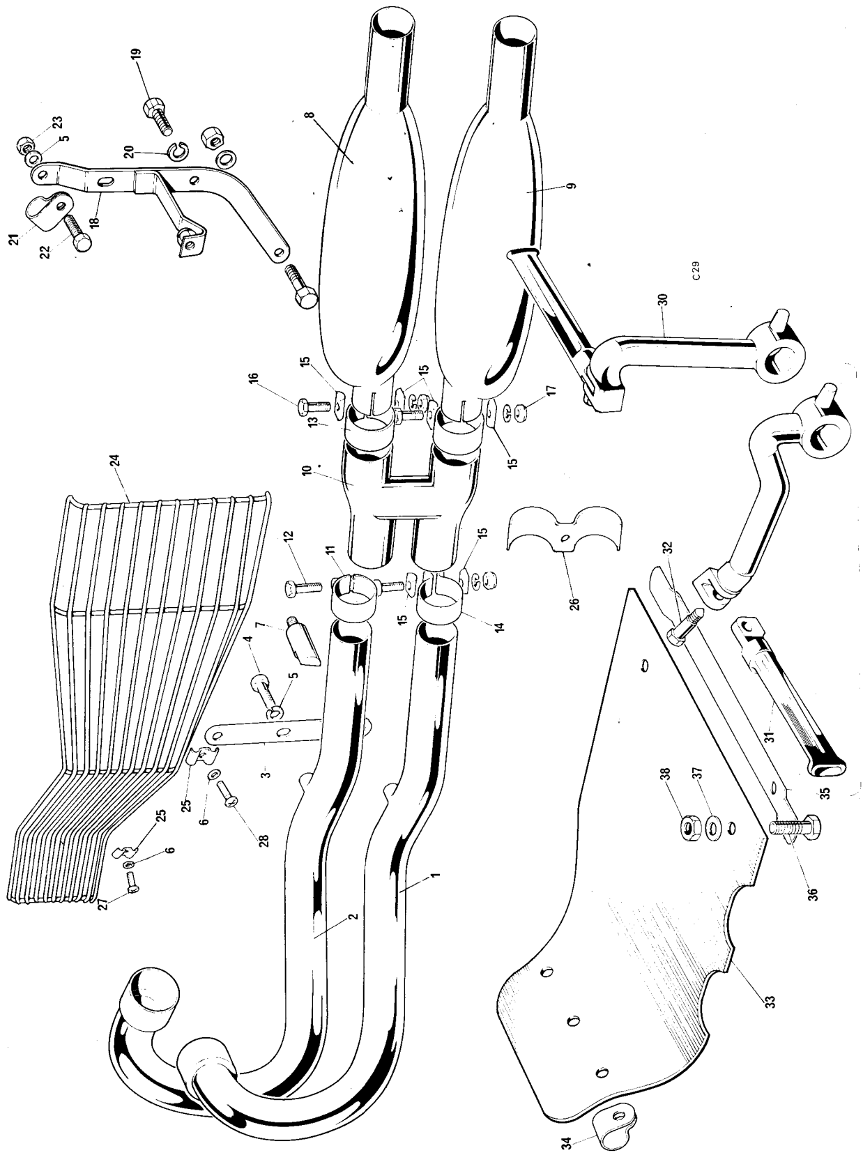
Fig. 17. EXHAUST PIPES, UNDERSHIELD AND FOOTPEGS (T100C)
