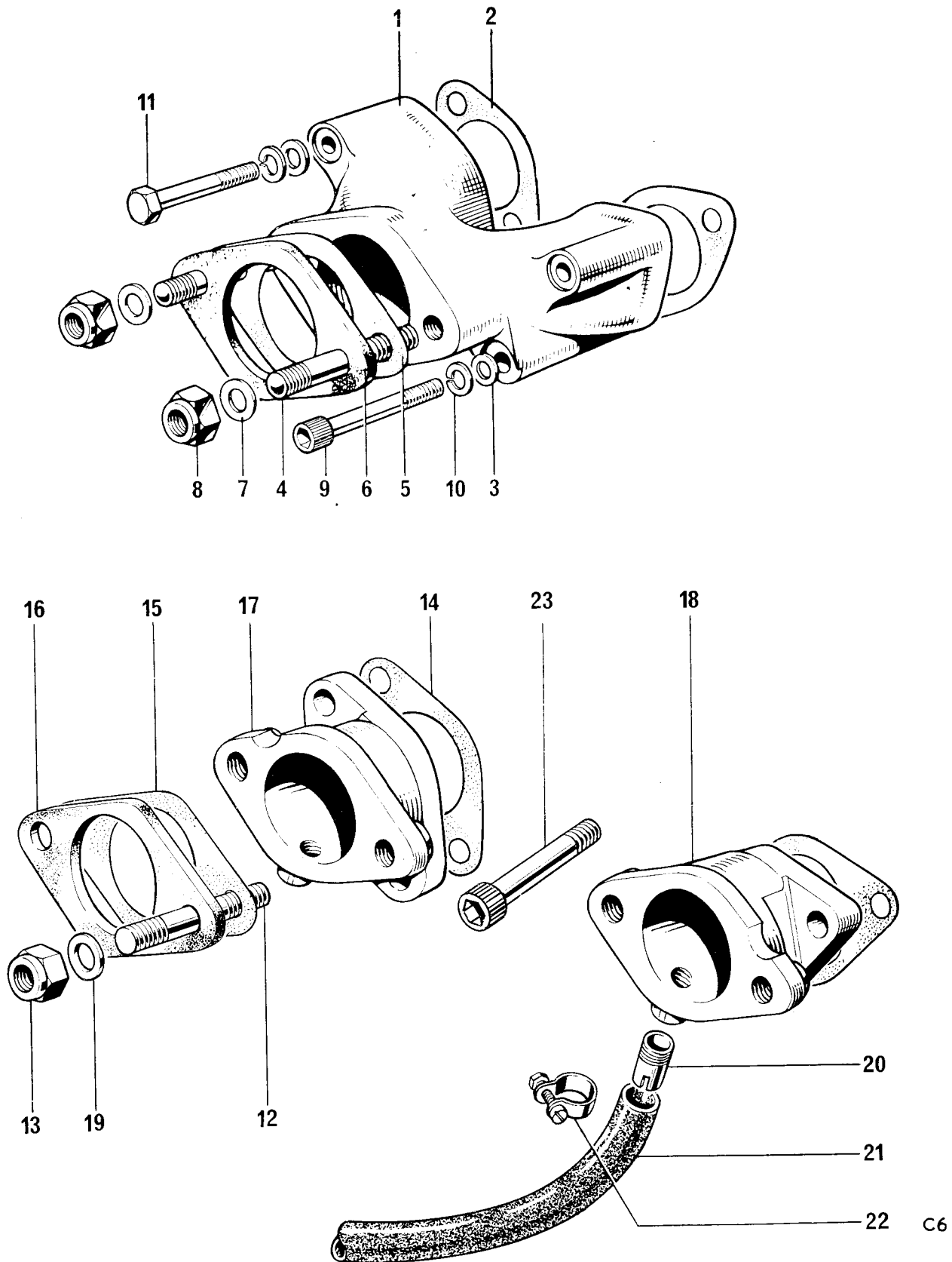
Fig. 4. INLET MANIFOLDS
