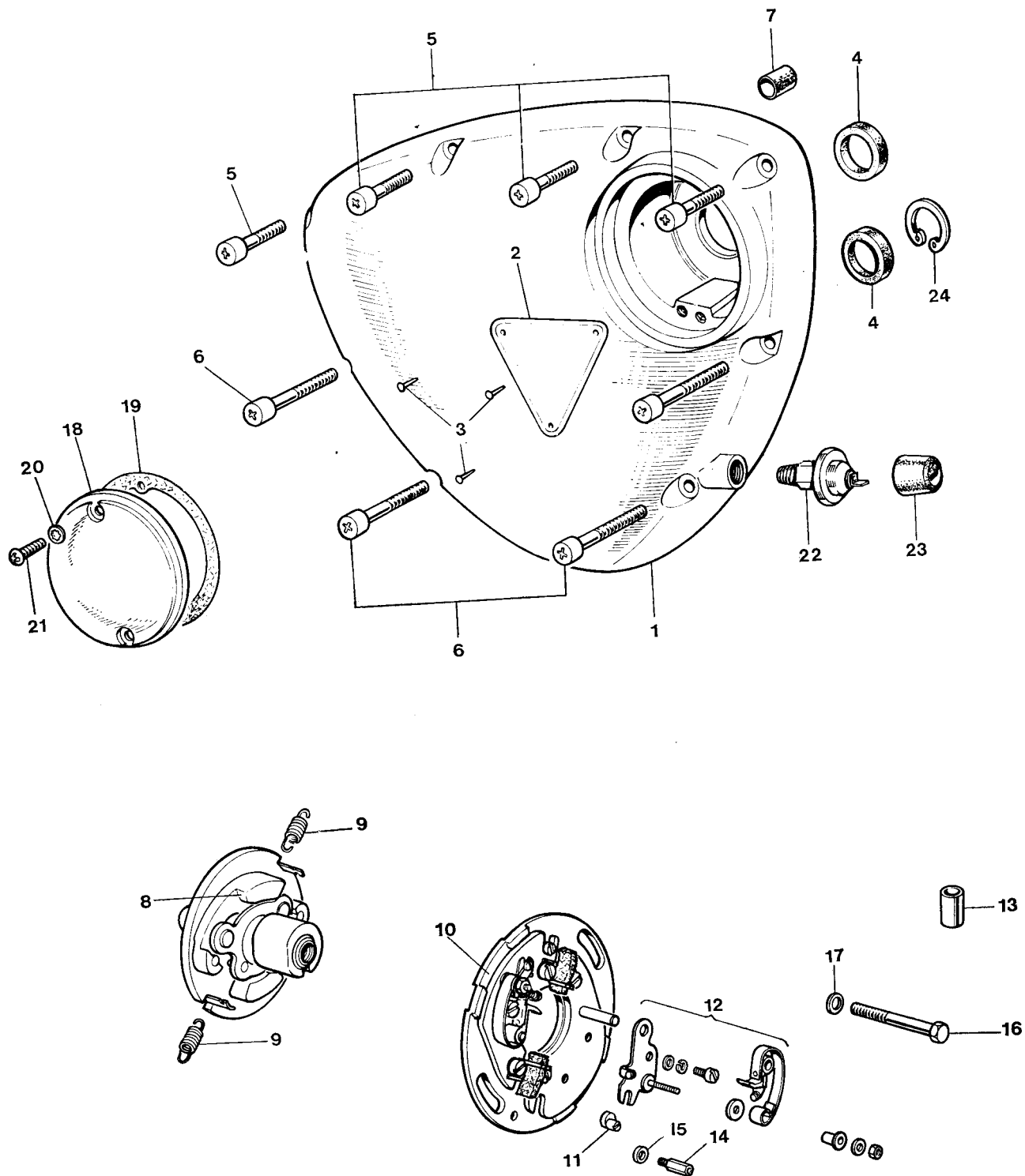
Fig. 8. TIMING COVER AND CONTACT BREAKER
