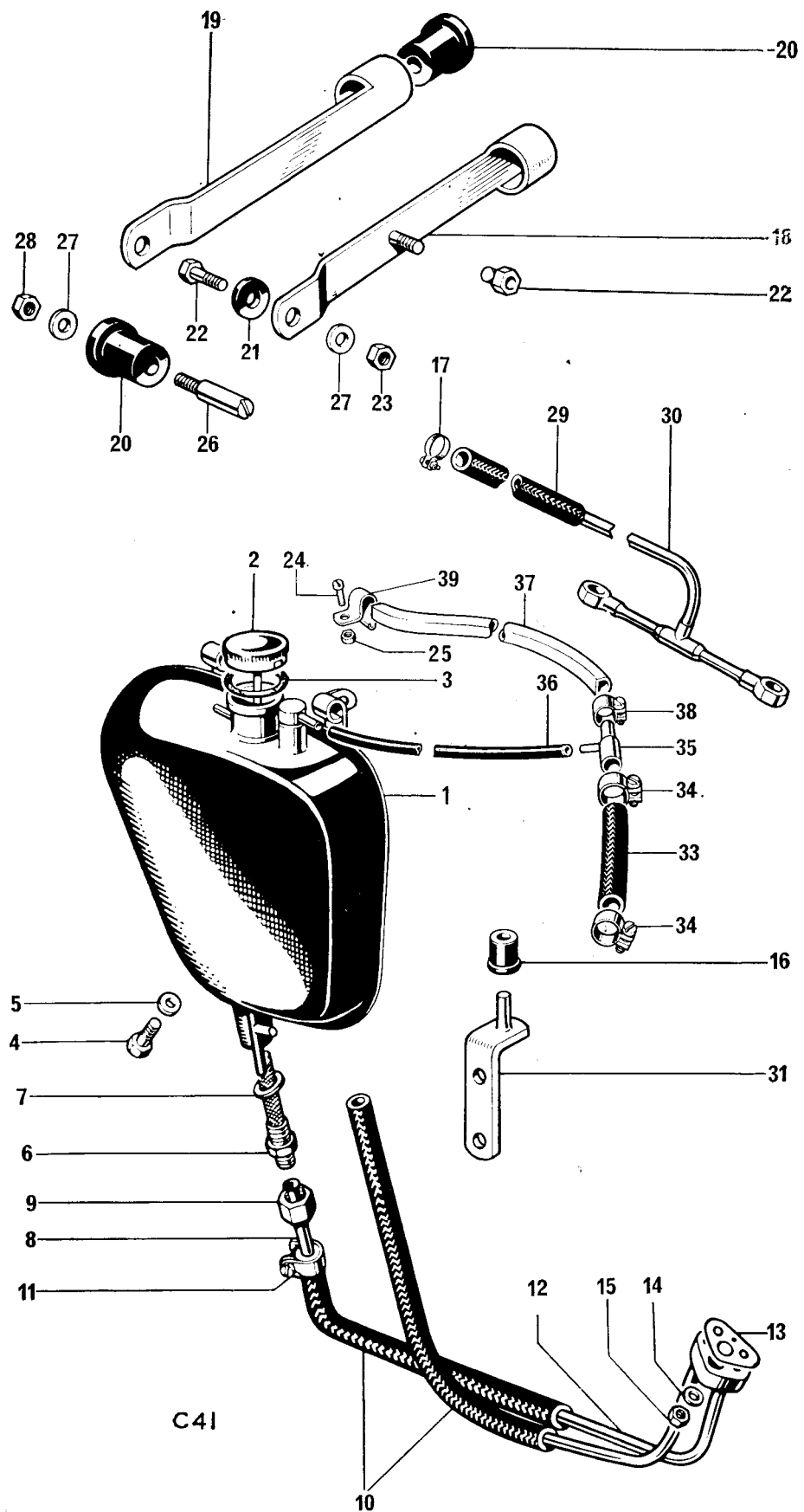
Fig. 28. OIL TANK
