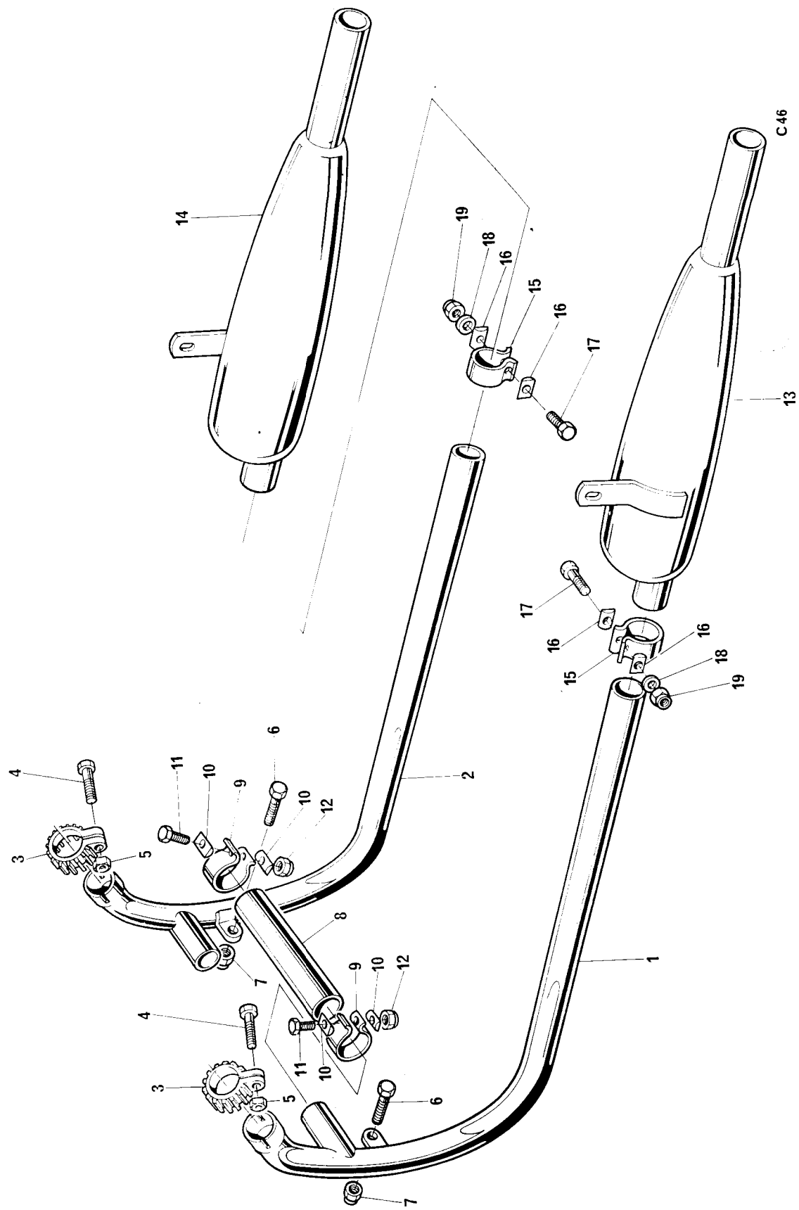
FIG. 15. EXHAUST SYSTEM
